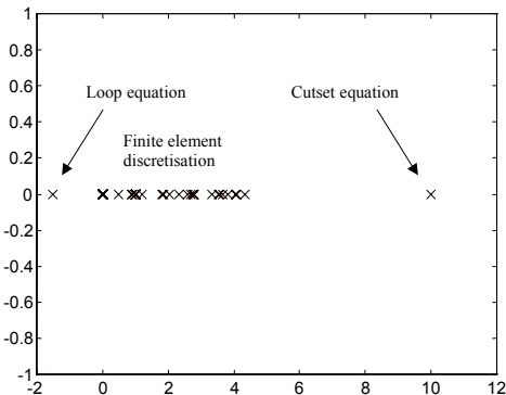
Fig. 1. Spectrum of a benchmark system matrix.
