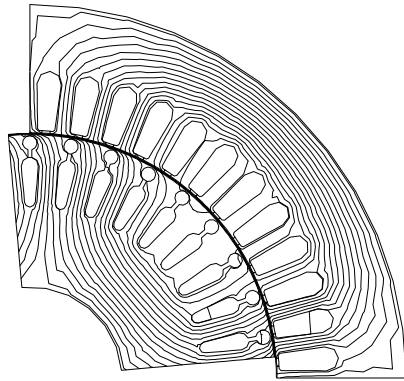
Fig. 3. Magnetic flux lines of the induction motor.
