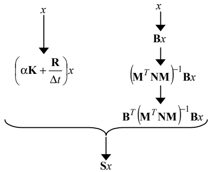
Fig. 2. Implicit multiplication procedure for \mathbf{Sx} .
