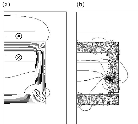
Fig. 10: Magnetic field distribution in an electromagnet, obtained by using a five-neuron (a) optimised and (b) non-optimised perceptron for the BH -characteristic of the armature.
