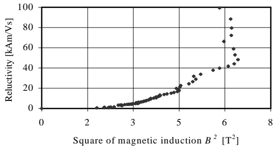
Fig. 2: Measured magnetisation curve of the ferromagnetic material in Fig. 1, in terms of v and B^2 .
