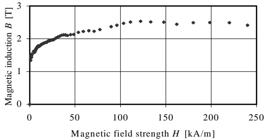
Fig. 1: Measured magnetisation curve of the ferromagnetic material with a carbon content of 0.55 %, in terms of B and H .
