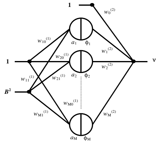
Fig. 3: Schematic view of a biased one-input one-output two-layer perceptron.
