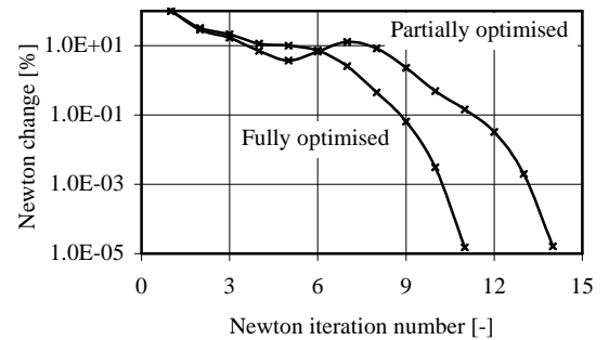
Fig. 11: Convergence of the Newton-method, obtained by using a five-neuron partially-optimised and fully-optimised perceptron for the BH -characteristic of the armature.
