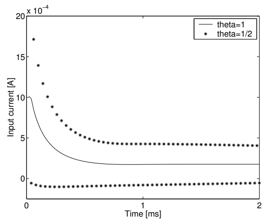
Fig. 7. Ion current through the wire for the Crank-Nicolson and the implicit schemes.
