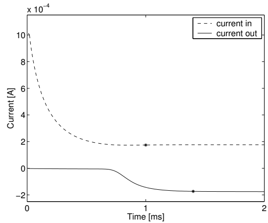
Fig. 2. Ion current flowing through the wire (in) and the plate (out); the '*' marks the point where the current has reached 99% of its steady state value.
