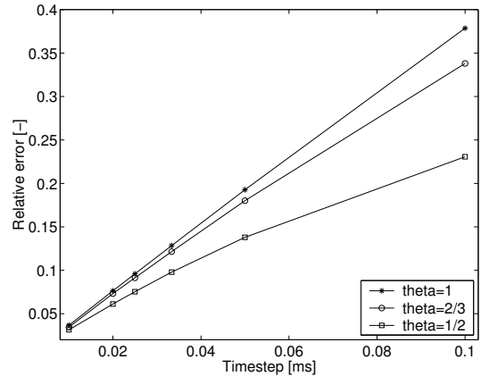
Fig. 6. Comparison of the relative error of the time schemes.
