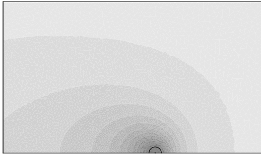
Fig. 4. Repartition of the charge density \rho_i at steady state, ranging from -5 \cdot 10^{-4} Cb/m 3 (black) to 0 Cb/m 3 (white).
