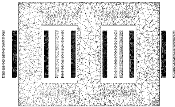
Fig. 7. Mesh used for thermal model; thin layer elements are put between the individual foils or anisotropic material is used.
