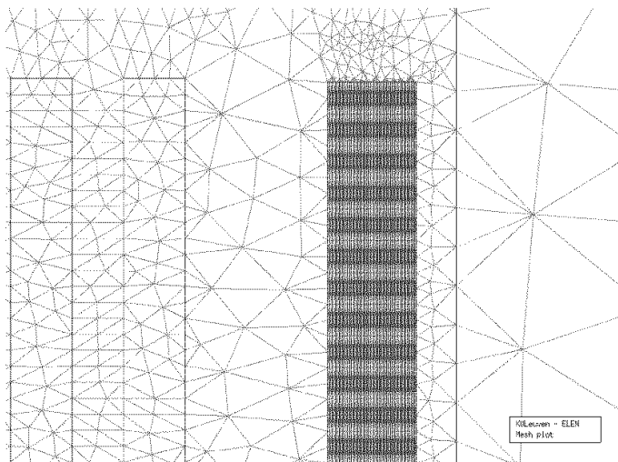
Fig. 3. Detail of the FEM mesh showing the fully meshed foil conductors.
