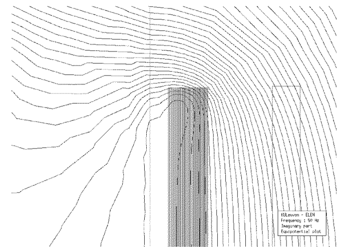
Fig. 5. Detail of the leakage flux (imaginary component); the field lines passing through the foil conductors in the top of the coil are associated with additional eddy currents and losses at that location.
