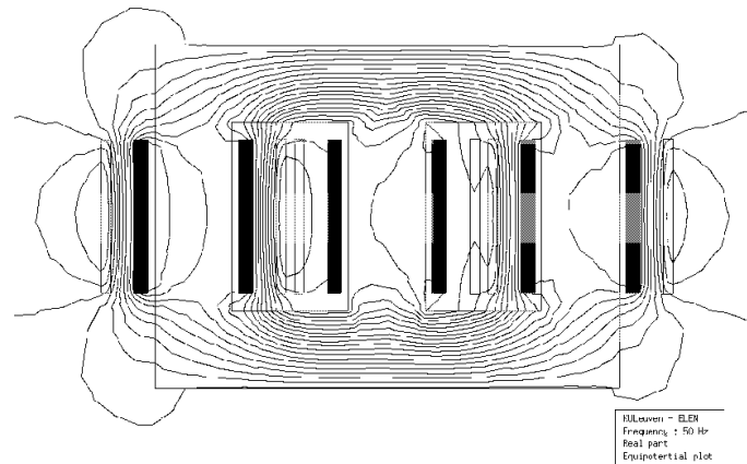
Fig. 4. Real part of the final magnetic field solution of a simulated short circuit test.
