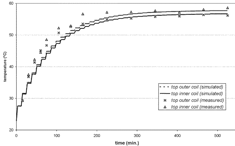
Fig. 9. Comparison of measured and calculated heating of the transformer in a short circuit situation. The temperature near the tops on the outer side is measured optically.
