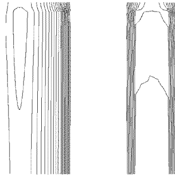
Fig. 8. Isothermal lines of the upper part of a coil set; on the left the foil conductor; on the right the wire coil. The hot spot is visible in the top of the foil pack.
