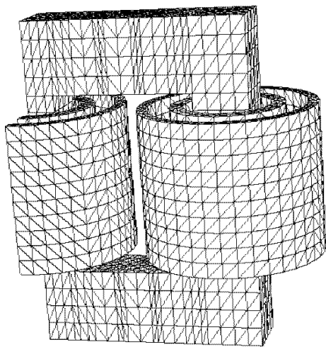
Fig. 2. 3D model used to determine the circuit parameters; the foil conductors are modeled as a solid block.
