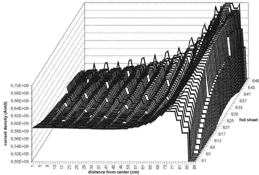
Fig. 6. Current density distribution in the 50 secondary foils, outside the core frame. Though there is a slight difference between the upper part and lower part of the coil, only the density in the (hotter) upper part is plotted; the foils closest to the core, having more eddy currents, are plotted in the background.
