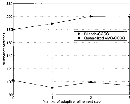
Fig. 2. Number of iterations of the block Jacobi and generalized algebraic multigrid schemes versus the number of adaptive refinement step.
